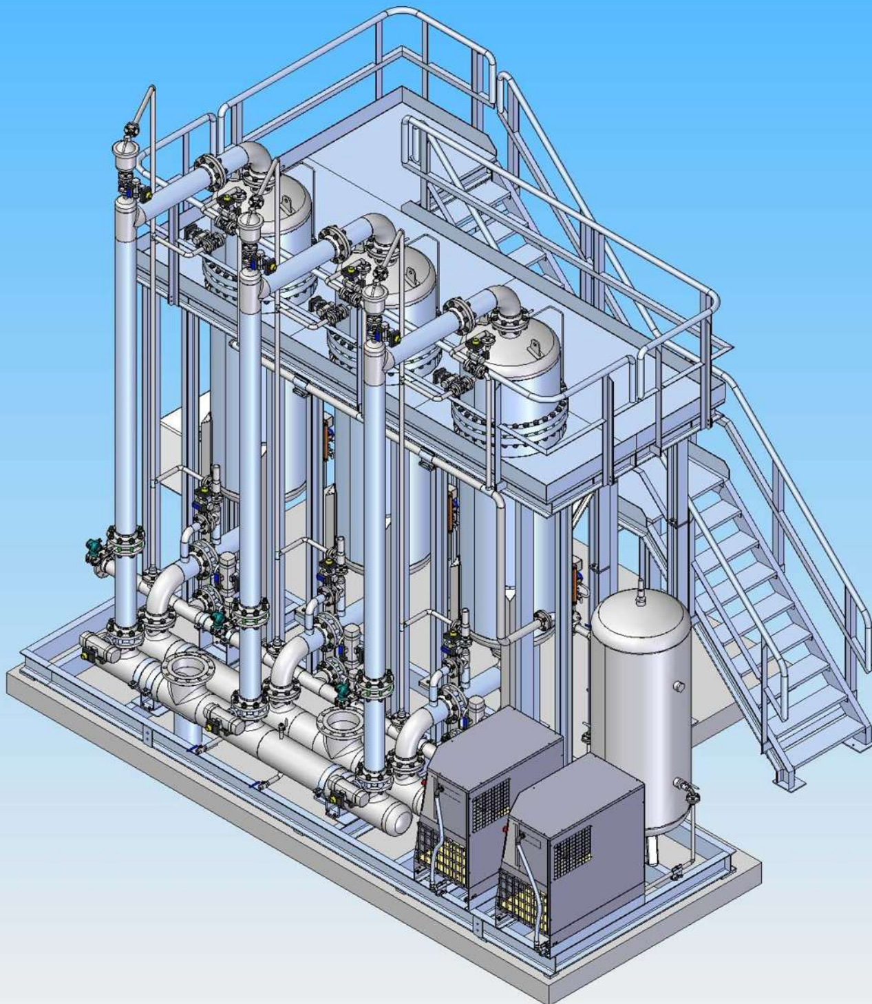
Equipment for a combined cycle power plant in Germany
